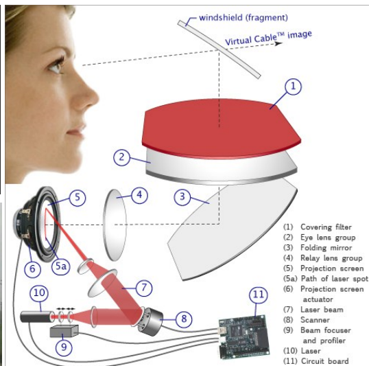
Fig. 3 Hardware components the Virtual Cable™ display (illustration)
