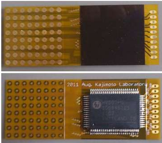
Fig. 2 Flexible electrode unit with 64 electrodes and 1 driver IC.
