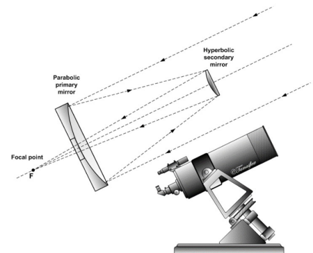
Cassegrain reflector (Wikipedia)
