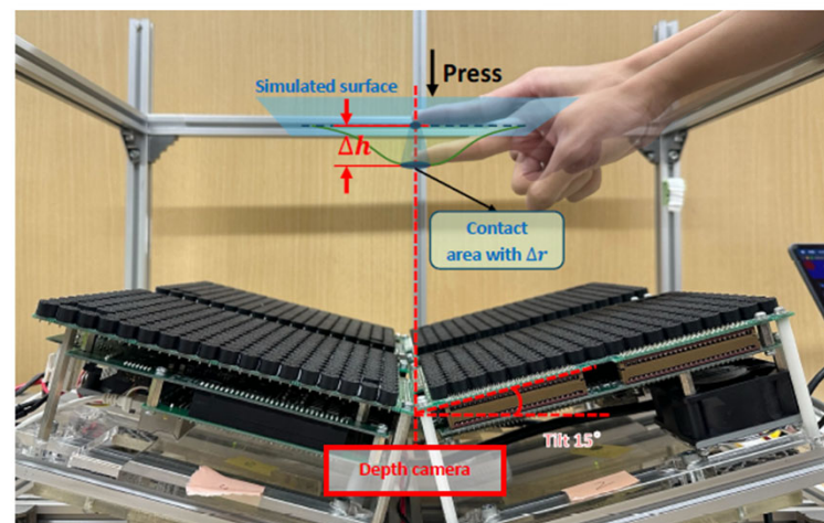
Fig. 5. System setup of the proposed method. Four AUTDs are deployed with a tilt angle of 15°.
