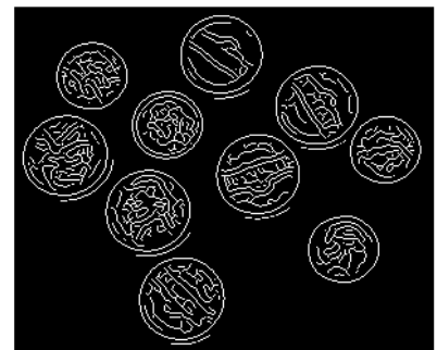
Canny
